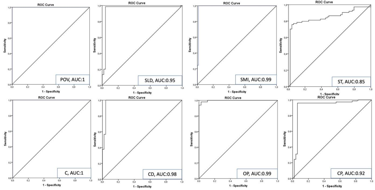
Supplementary Fig. S1. ROC curves for eight variables. Name of the variable and AUC values are shown in the blue boxes at right bottom of each ROC curves. ROC, receiver operating characteristic; AUC, area under the curve; POV, percent object volume; SLD, structure linear density; SMI, structure model index; ST, structure thickness; C, connectivity; CD, connectivity density; OP, open porosity; CP, closed porosity.
